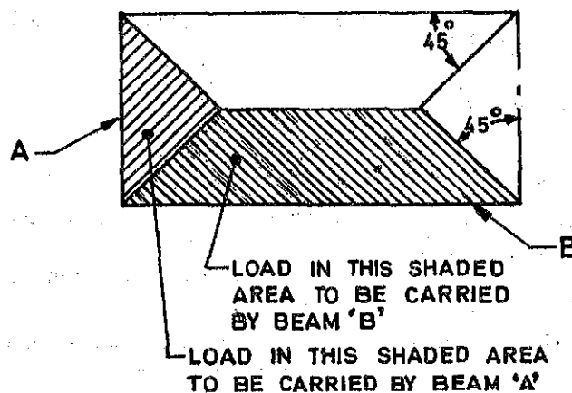
FIG. 7 LOAD CARRIED BY SUPPORTING BEAMS
