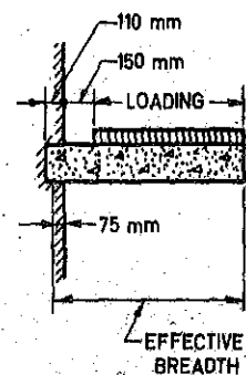
FIG. 19 LOADING ON STAIRS BUILT INTO WALLS
